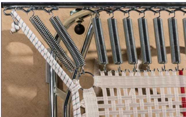
Tension provided by 32 springs
